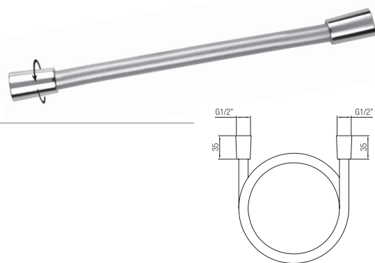
Flessibile doccia SILVER. SILVER flexible hose.
