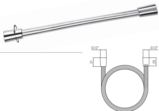
Flessibile doccia CHIC. CHIC flexible hose.
