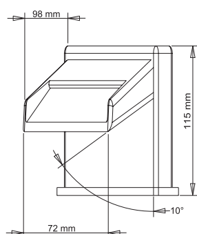
Bocca vasca/lavabo cascata. Bath/basin spout waterfall jet.
